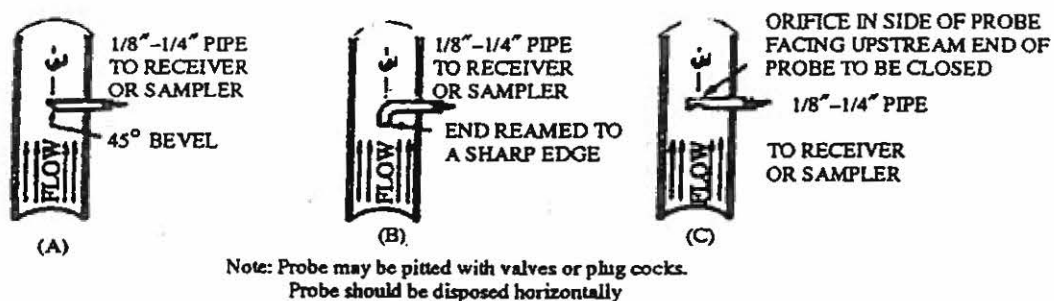
Figure 4. Probes for Continuous Sampling
