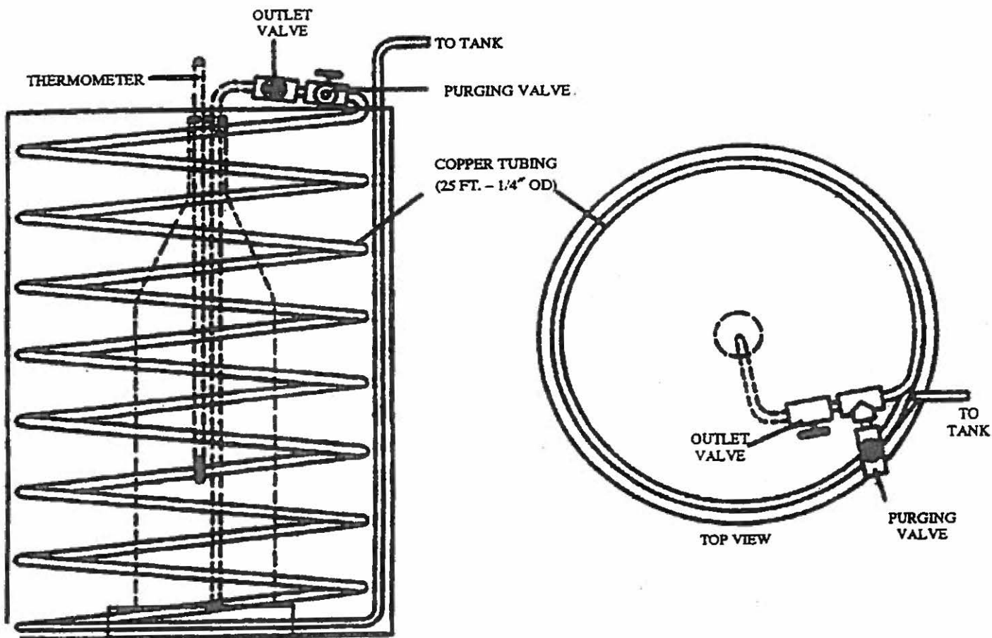
Figure 5. Cooling Bath
